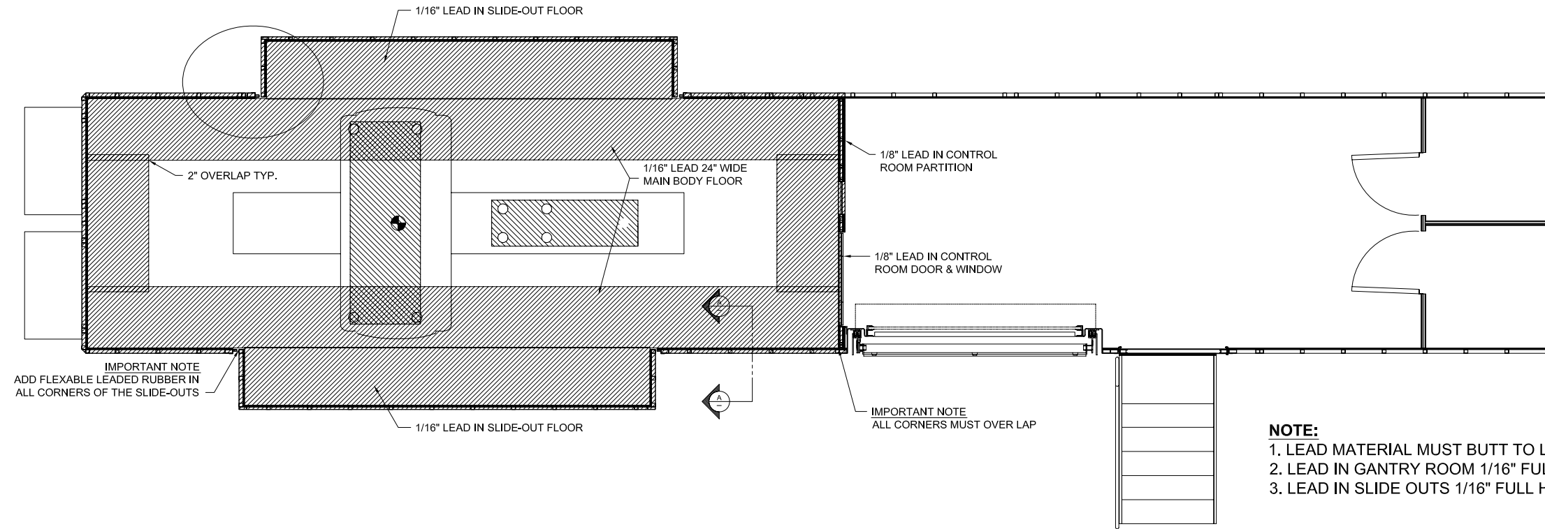
PLAN VIEW
