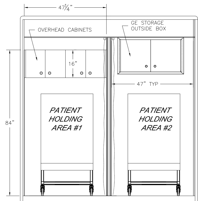
SECTION "A-A"
