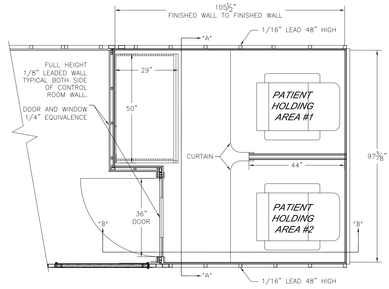
PLAN VIEW OF DISPENSING AREA PARTITION WALL
